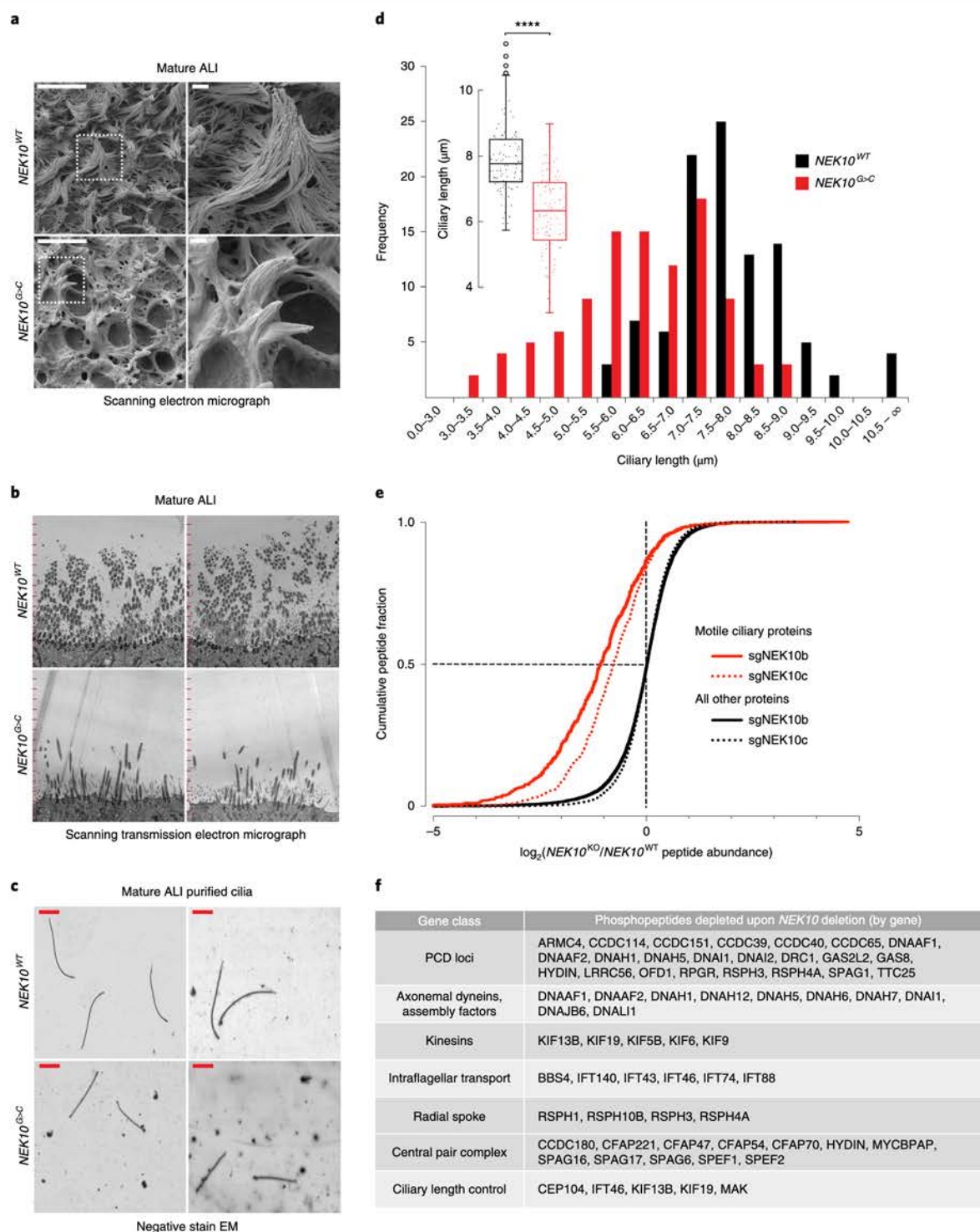
Fig. 4 | NEK10 regulates ciliary length through widespread effects on the ciliary proteome. a , SEMs of mature ALI cultures of the indicated genotype, representative of three independent ALI differentiations. The dashed boxes mark full resolution regions shown in the right panels. Scale bars, 10 μm (left panels) or 1 μm (right panels). b , STEMs of mature ALI cultures of the indicated genotype after embedding and sectioning orthogonal to the epithelial surface, representative of three independent ALI differentiations. Tick marks are spaced at 1 μm. c , Representative negative stain electron microscopy grids prepared from purified cilia of the indicated genotypes, representative of two independent ALI differentiations. Scale bar, 1 μm. d , Histogram of ciliary length from purified cilia of the indicated genotypes. n = 101 for NEK10 WT and n = 102 for NEK10 G-C , pooled from two independent ALI differentiations. The inset shows a box and whisker plot of these data, in which the center line indicates the median, the box bounds the 25th and 75th percentiles, the whiskers indicate 1.5 times the interquartile range, and the circles indicate outliers. e , Cumulative distribution of phosphopeptides by log 2 [fold change]. Previously identified motile ciliary proteins are shown in red, and all other detected proteins are shown in black. sgNEK10b and sgNEK10c are independently targeting guide RNAs validated in Extended Data Fig. 3d. f , Table of ciliary genes by functional class showing phosphopeptides that were depleted more than twofold upon NEK10 deletion. WT, wild type. **** P \leq 0.0001 .
